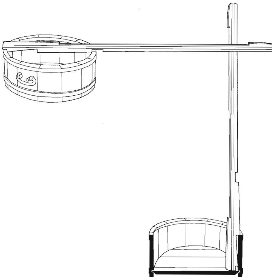
Figure 2. Diagram showing the use of the Inverkeithing gauge to check the depth and diameter of a firloft measure.
