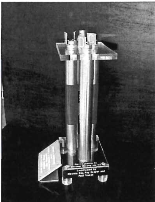
Calculable Capacitor – photo courtesy of Monash University
