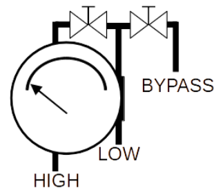
Figure 1. Typical Mechanical Backflow Test Kit
